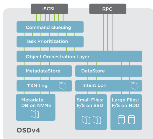
PanFS Intelligent Multi-tier Architecture
