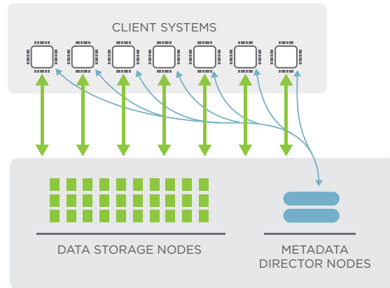
PanFS Parallel File System
